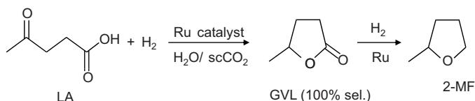
Fig. 12. Hydrogenation of levulinic acid to \gamma -valerolactone.
